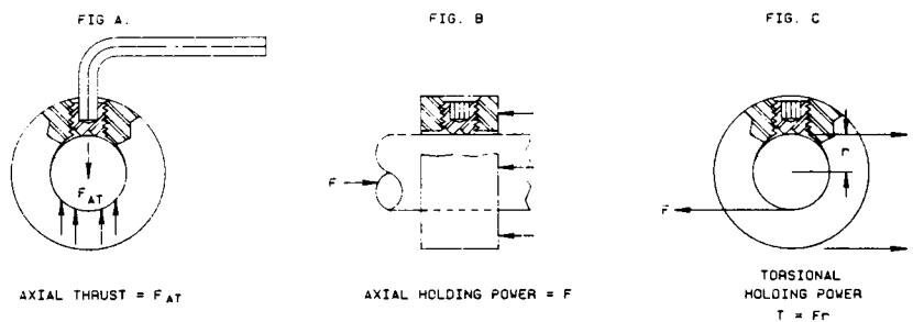
SET SCREW HOLDING POWER
